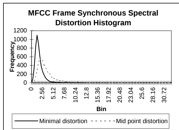
Figure 1: Histogram of spectral distortion values.
